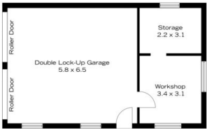
Ground Floor
